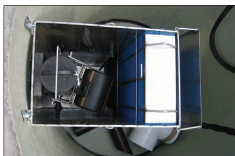
ecoLine™-b coalescing outlet structure with automatic shutoff valve
