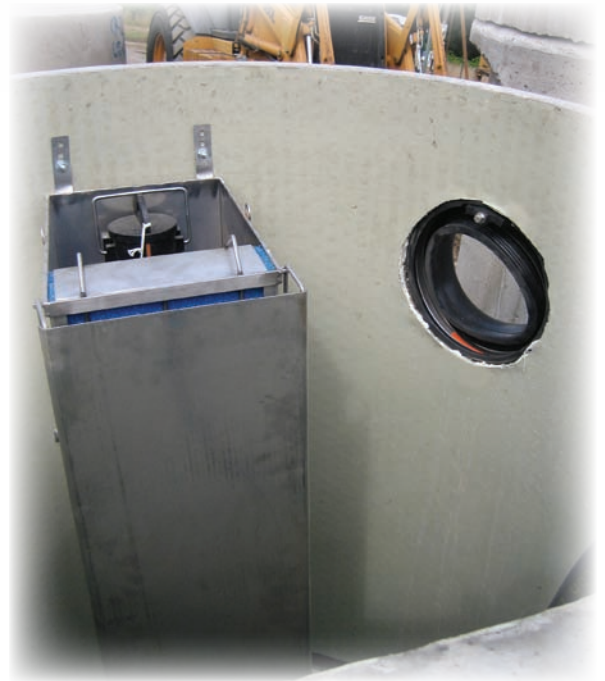
ecoLine™-b coalescing unit installed inside a lined precast concrete structure
